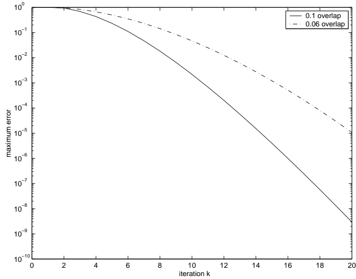
Figure 7: Two dimensional model problem with four subdomains, algorithm in the super-linear convergence regime for T = 0.05 .
