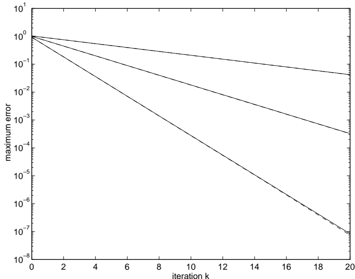
Figure 3: Theoretical and measured decay rate of the error for two subdomains and three different sizes of the overlap.
