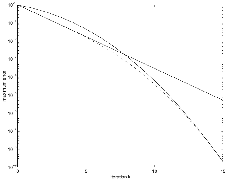
Figure 5: Transition from the linear to the superlinear convergence regime. The convergence rate of the algorithm is first dominated by the linear convergence regime and after some iterations by the superlinear convergence regime.
