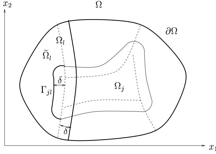
Figure 2: Information for \Omega_j from the neighboring subdomain \Omega_l is only used from within \tilde{\Omega}_l .
