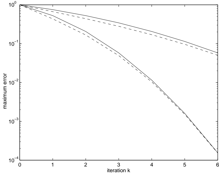
Figure 4: Superlinear decay of the error for a small time interval and two different sizes of overlap.
