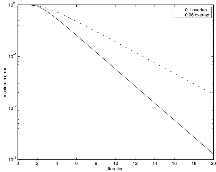
Figure 6: Two dimensional model problem with four subdomains, algorithm in the linear convergence regime for T = 3 .
