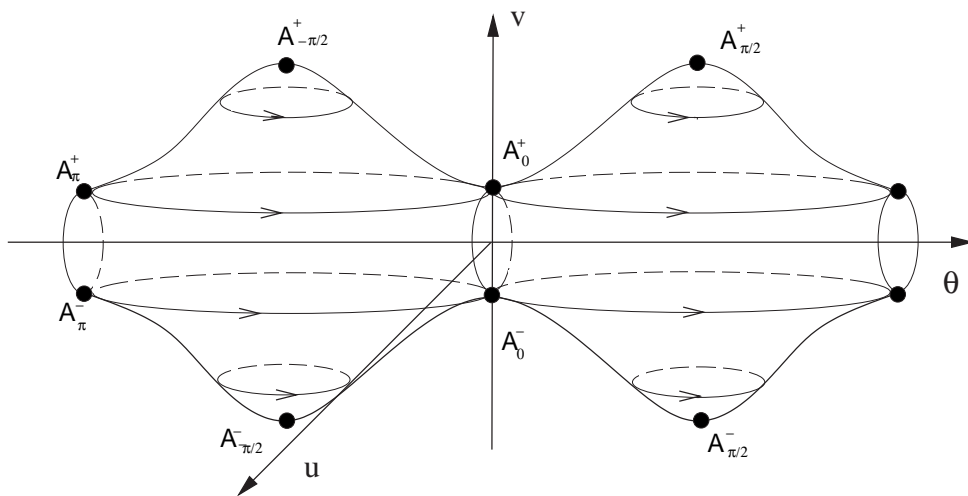
Figure 1: The flow on the collision manifold, which is formed by periodic orbits, eight equilibria, and eight heteroclinic orbits.
