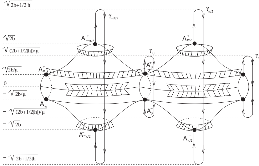
Figure 2: The flow can reach the collision manifold at the equilibria or at any of the periodic orbits. There are four heteroclinic orbits \gamma_{-\pi/2}, \gamma_0, \gamma_{\pi/2}, \gamma_{\pi} connecting respectively A_{-\pi/2}^+ with A_{-\pi/2}^- , A_0^+ with A_0^- , A_{\pi/2}^+ with A_{\pi/2}^- , and A_{\pi}^+ with A_{\pi}^- .
