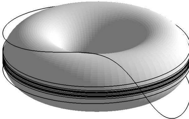
Figure 3: An homoclinic orbit to p_0 lying on the homoclinic manifold. This orbit spirals out of the equator of the collision manifold and then spirals back to it.
