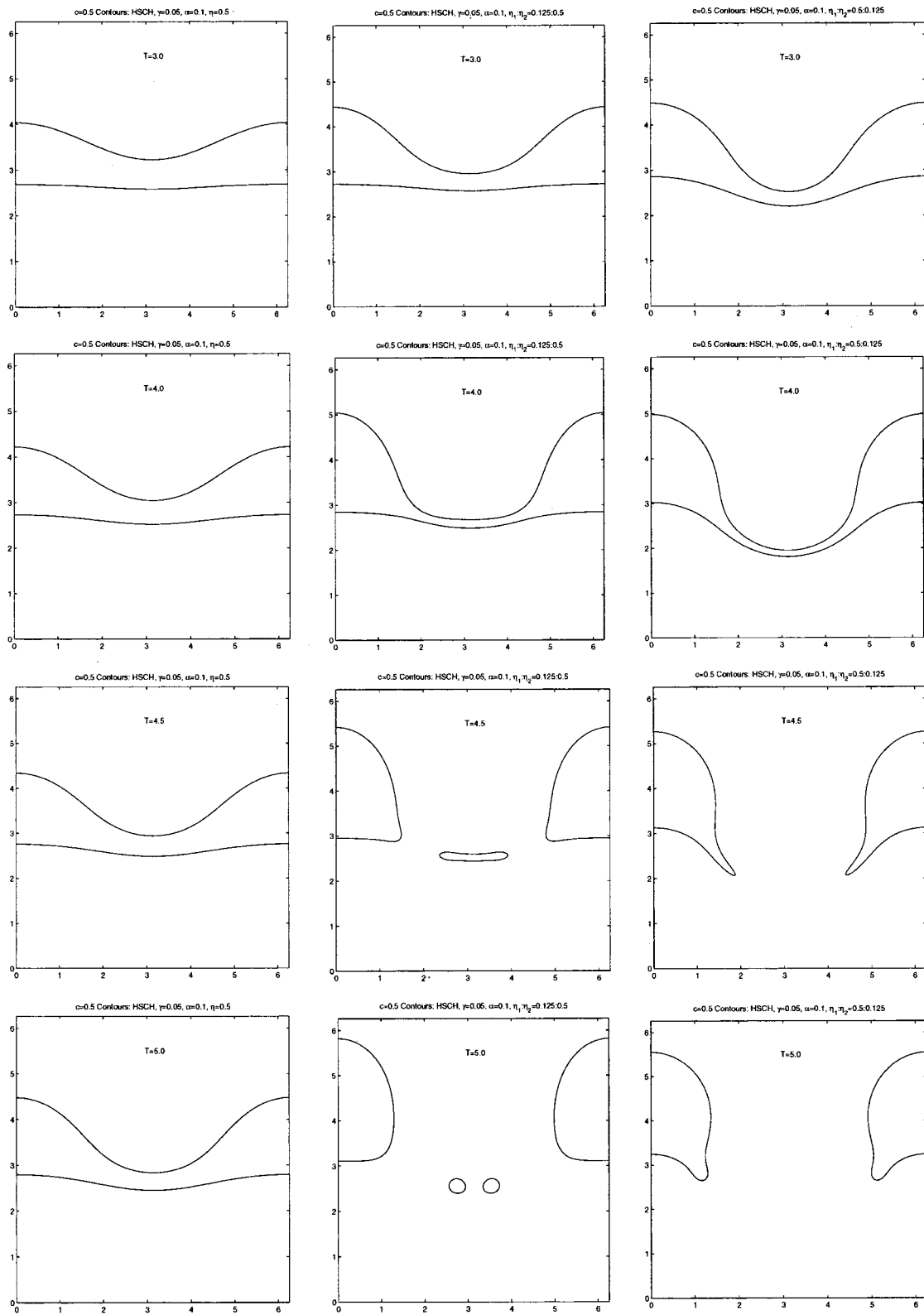
FIG. 18. The effect of viscosity difference on the c = 0.5 contours in the HSCH model. \gamma = 0.05 , \alpha = 0.1 and |\mathbf{B}| = 25 . Left-most column, \eta_1 = \eta_2 = 0.5 ; center column, \eta_1 = 0.125 , \eta_2 = 0.5 ; right-most column \eta_1 = 0.5 , \eta_2 = 0.125 .
