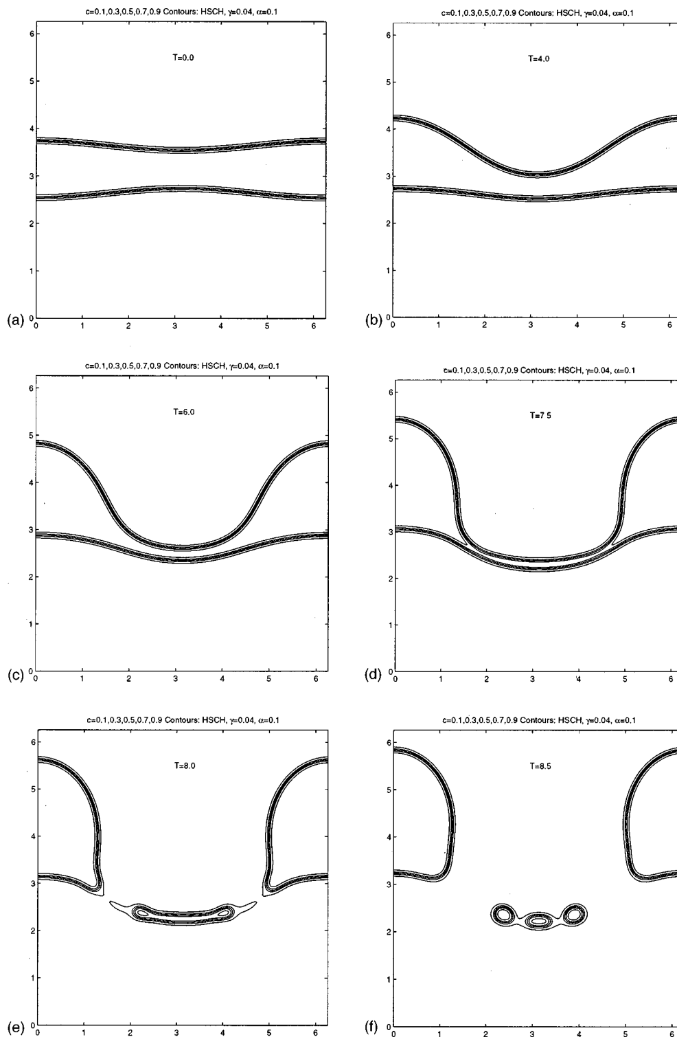
FIG. 4. Contours of c for the HSCH model with |B|=25 , \alpha=0.1 , and \gamma=0.04 . (a) t=0 ; (b) t=4.0 ; (c) t=6.0 ; (d) t=7.5 ; (e) t=8.0 ; (f) t=8.5 . The 0.1, 0.3, 0.5, 0.7, and 0.9 contours are shown.
