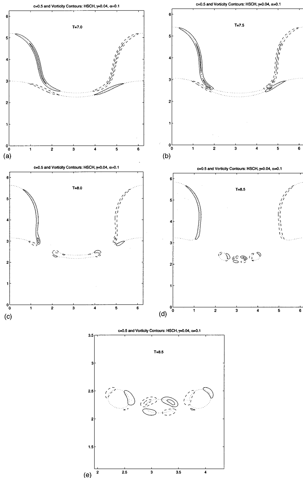
FIG. 6. Vorticity and concentration contours for HSCH model from Fig. 4. Dotted curve, c=1/2 contour; solid curves, positive vorticity \omega=(0.25,0.75) \cdot \omega_{\max} ; dashed curves, negative vorticity \omega=(0.25,0.75) \cdot \omega_{\min} . (a) t=7.0 ; (b) t=7.5 ; (c) t=8.0 ; (d) t=8.5 ; (e) t=8.5 close-up of satellite drop region.
