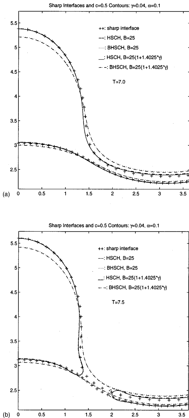
FIG. 20. Close-up of comparison of modified Bond number HSCH $c=0.5$ contours with the sharp interface result. $\gamma=0.04$ and $\alpha=0.1$. Sharp interface (+ curves); HSCH and BHSCH models with $|B|=25$ (dashed and dotted curves, respectively); HSCH and BHSCH models with $|B|=25(1+1.4025\gamma)$ (solid and dotted-dashed curves, respectively). (a) $t=7.0$; (b) $t=7.5$.
