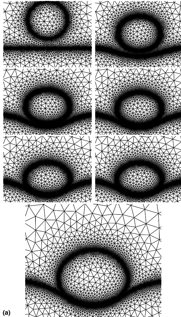
Fig. 3. 2D simulation (a) of drop impact in Stokes flow onto an interface under gravity ( \lambda = 1 , Bo = 0.8 ). Mesh parameters h_0/a = 0.5 , s = 0.3 , h_1/a = 0.0125 . Drop-to-domain size ratio 0.1. Time \bar{t} = t/(\mu a/\sigma) = 0, 5, 10, 15, 40, 55 . Bottom: close-up at \bar{t} = 55 , the onset of coalescence. Same as (a) but for mesh parameter h_1/a = 0.05 corresponding to a coarser mesh (b). Time \bar{t} = 0, 5, 10, 15, 20 and 25. Rapid coalescence is erroneously predicted. Minimum distance \bar{w} = w/a between the drop and interface (c) for different mesh resolutions as a function of time (initially, \bar{w} = 0.5 ). Solid: From left to right, simulations for h_1/a = 0.05 as in (b), 0.035, 0.025 and 0.0125 as in (a). Dashed: exponential gap thinning behavior from lubrication theory (24). As h_1 is decreased, the simulation is more accurate and agrees with the theory down to smaller gap thicknesses w = O(h_1) .
