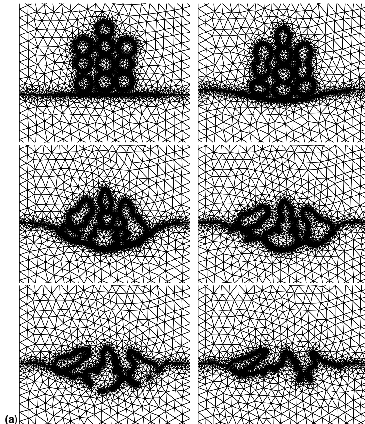
Fig. 4. Sedimentation under gravity and coalescence (a) of a system of 10 drops of fluid 1 onto a fluid/fluid interface separating fluid 2 (above the interface) from a reservoir of fluid 1 below the interface. The drops have slightly bidispersed sizes. Bond number Bo = 80 (based on the larger drop size) and viscosity ratio \lambda = 1 . Mesh parameters h_0/a = 1 , h_1/a = 0.075 and s = 1 . Times t/(\mu a/\sigma) = 0, 0.01, 0.05, 0.1, 0.15, 0.2 (left to right, top to bottom). Same as in (a) except the Bond number Bo = 0.8 (b). Times t/(\mu a/\sigma) = 0, 2.5, 5.0, 7.5, 10.0, 10.5 .
