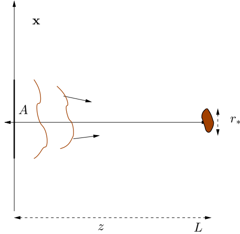
FIGURE 1. The time reversal procedure. A source emits a pulse in the plane z = L . The transmitted field is recorded and time reversed at the mirror of size A at z = 0 , and then sent back toward the source point. There it refocuses on a spot with the lateral size r_* . Medium heterogeneity typically enhances the refocusing resolution.
