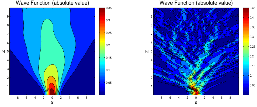
Figure 3: |\psi(z, x)| for one realization for \varepsilon_x = 10\sigma_I = 10 (left) and \varepsilon_x = \sigma_I = 1 (right), with R_0 = 0.25 . For the same reasons as in figure 2, |\psi(z, x)| on the left is close to the homogeneous solution, while it is random on the right.
