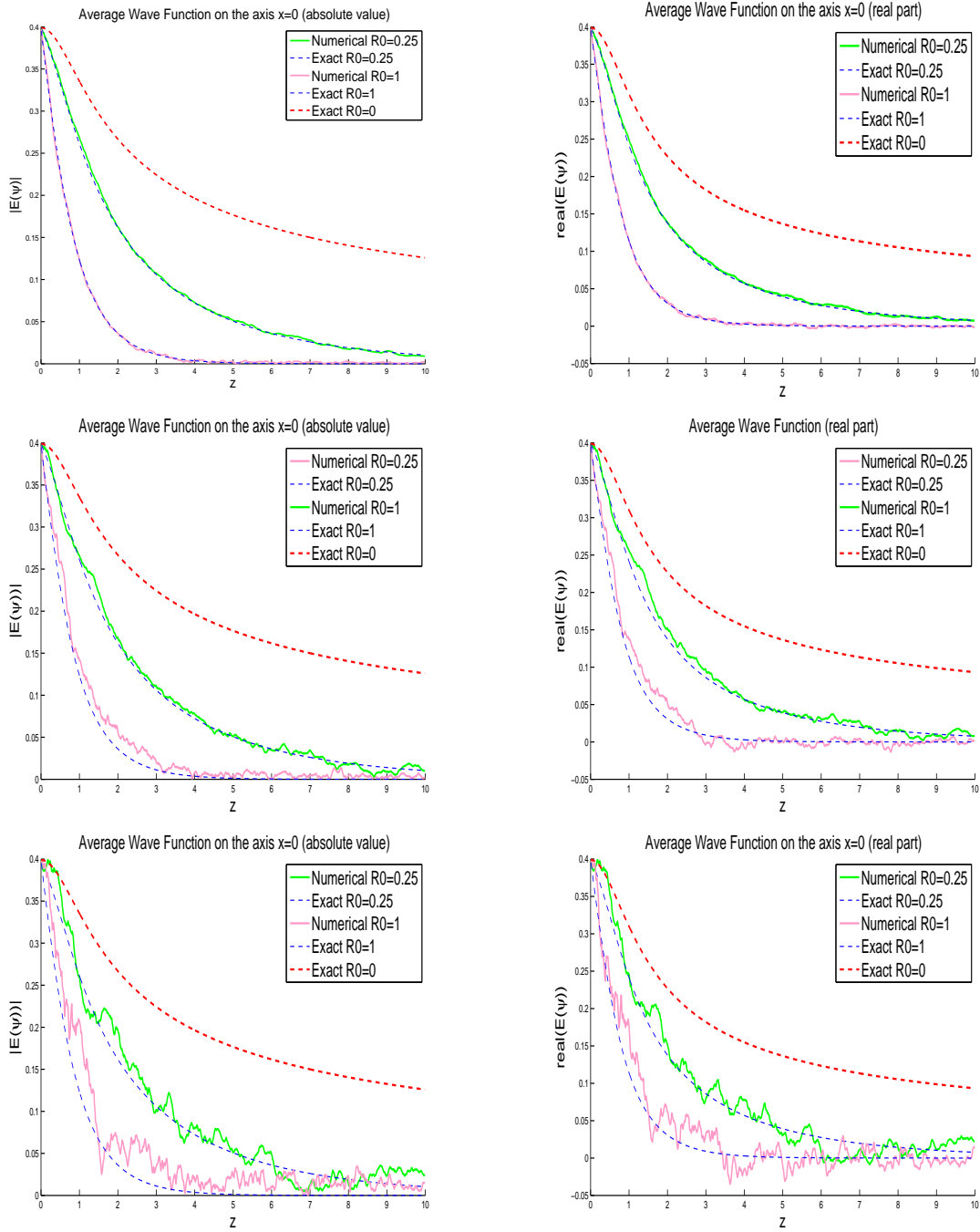
Figure 1: Average wave function on the axis x = 0 as a function of z , for N_r = 1000, 100, 10 , top to bottom, and R_0 = 0, 0.25, 1 . Left: absolute value, right: real part. Statistical instabilities are observed when N_r = 10 , while we have an almost perfect match when averaging is strong enough with N_r = 1000 .
