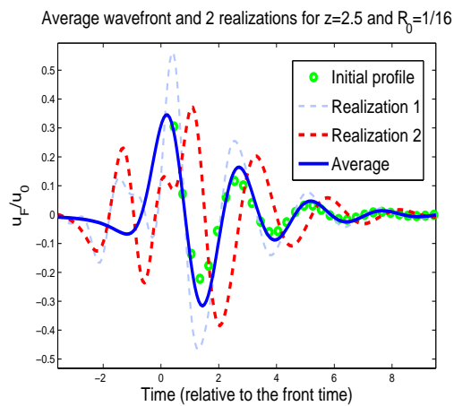
Figure 9: Average wavefront amplitude (solid line) at z = 2.5 as a function of t for R_0 = 1/16 , \sigma_I = \varepsilon_x = 1 , \delta = 0 and 2 realizations (dash lines). The initial profile \beta_2(t) (shifted appropriately) is represented by the circles. The absorption \eta is equal to 0.2. The qualitative behavior of the random wavefront is similar to the average wavefront.
