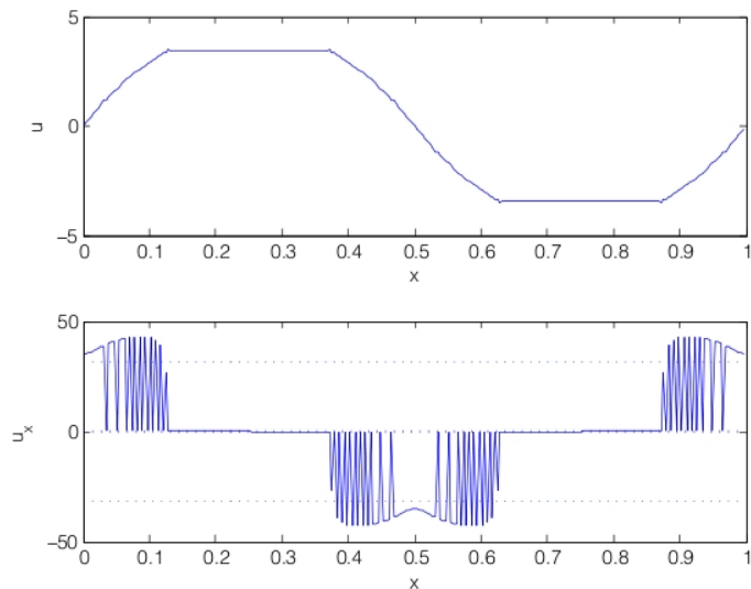
Fig. 3. Microstructured gradient for a typical solution of (13).
