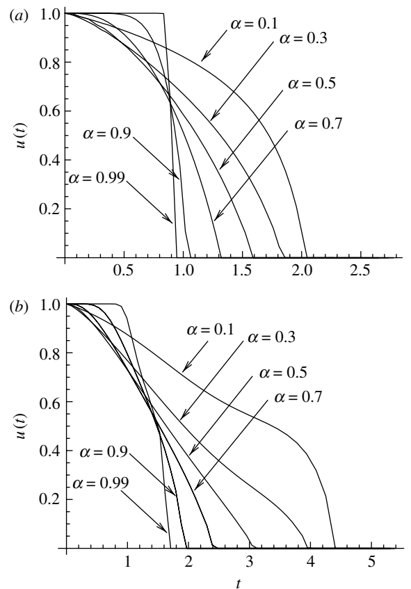
Figure 8. The optimal control found by the SQP method, for different values of \alpha < 1 , for (a) a one-step process and (b) a two-step process. The other parameters are a=2, \sigma=10, u_m=1, \mu=10^{-1} .
