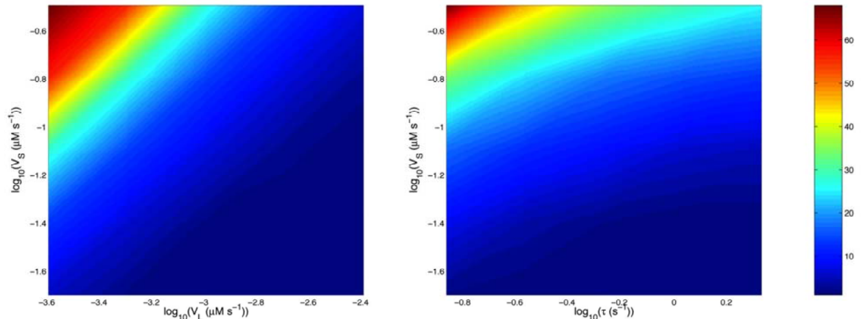
Supplemental Figure S10. Time for [S] to Reach Its Maximum
