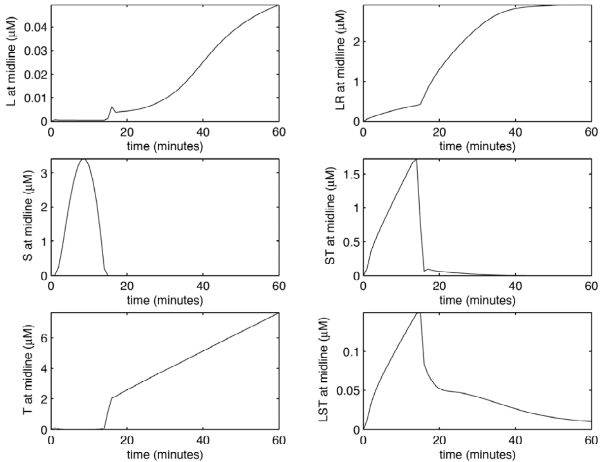
Supplemental Figure S9. Dynamic Behavior of the Full Model at the Dorsal Midline
