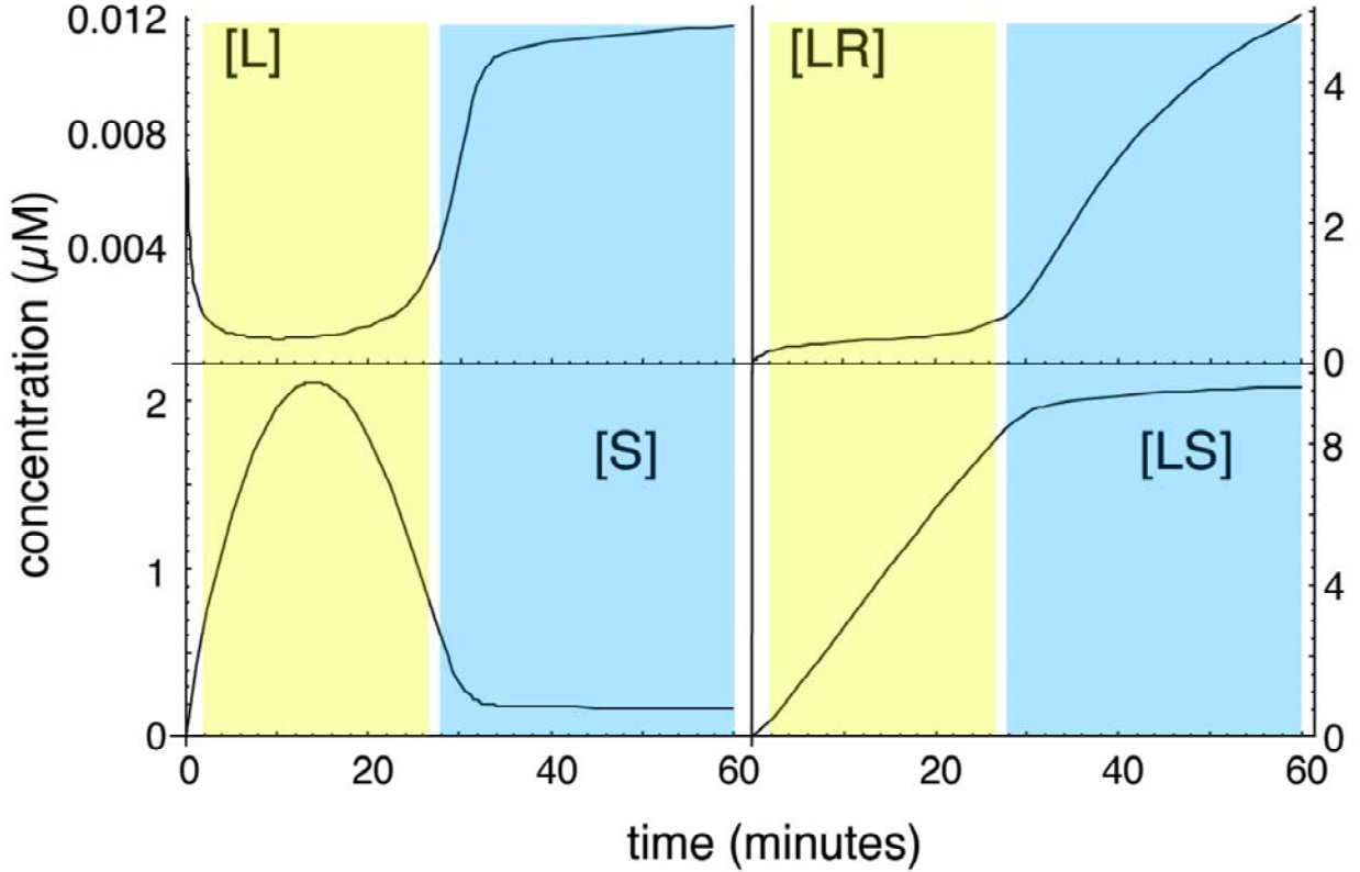
Supplemental Figure S8. Dynamic Behavior of a Simplified Space-Independent Model Equations 1-4 were solved numerically from 0 to 3600 s (1 hr). [L], [LR], [S], and [LS] are plotted in units of \mu\text{M} . Parameters were v_L = 6 \text{ nM} ; v_S = 10 \text{ nM} ; k_{\text{on}}R_0 = 0.5 \text{ s}^{-1} ; k_{\text{deg}} = 0.001 \text{ s}^{-1} ; j_{\text{on}}R_0 = 5 \text{ s}^{-1} ; j_{\text{off}} = 3 \times 10^{-4} \text{ s}^{-1} ; \tau = 0.001 \text{ s}^{-1} . Note the distinct “plateau” and “jump” phases, which are shaded in yellow and blue, respectively.
